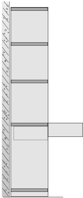
Lift tray for W3 side panel shelf unit – (B3WTAL...48) flush finish with 2.8 cm shelf
